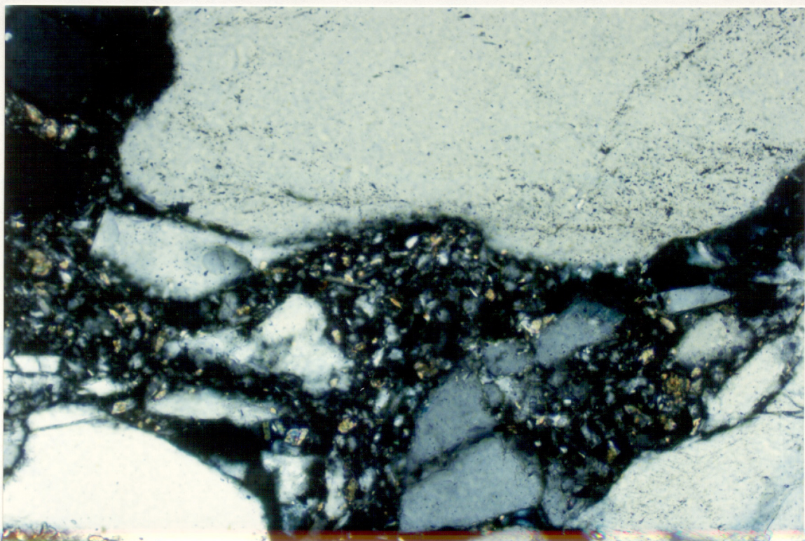
Figure 9: SWC 22, 2945m, 2mm, PPL Thin bed of opaques (O) and very fine-grained carbonate (A). The opaque grain marked shows a finely punctate texture.
