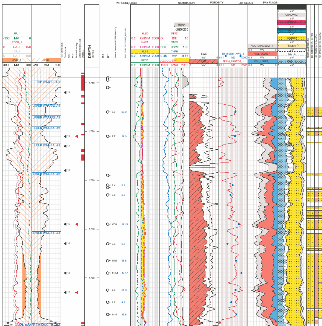
Figure 3.6.4 – c : Casino-1 Log Analysis (Waarre A Reservoir)
