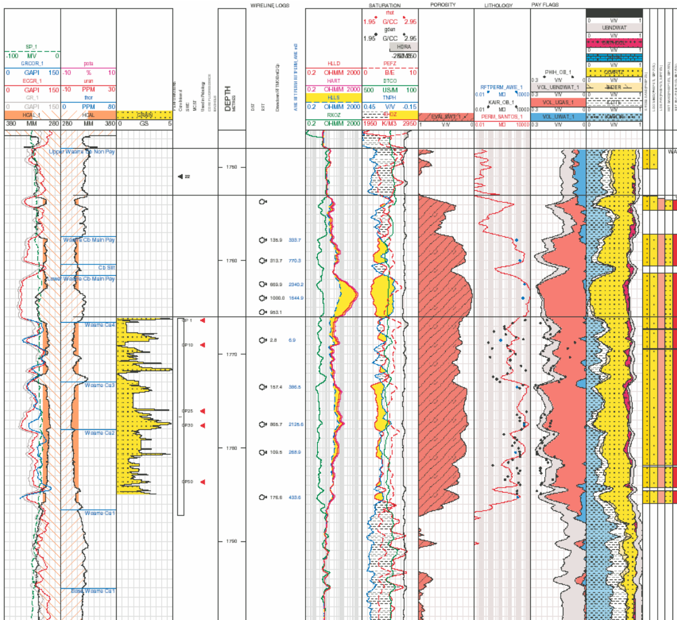
Figure 3.6.4 – d : Casino-2 Log Analysis (Waarre C Reservoir)
