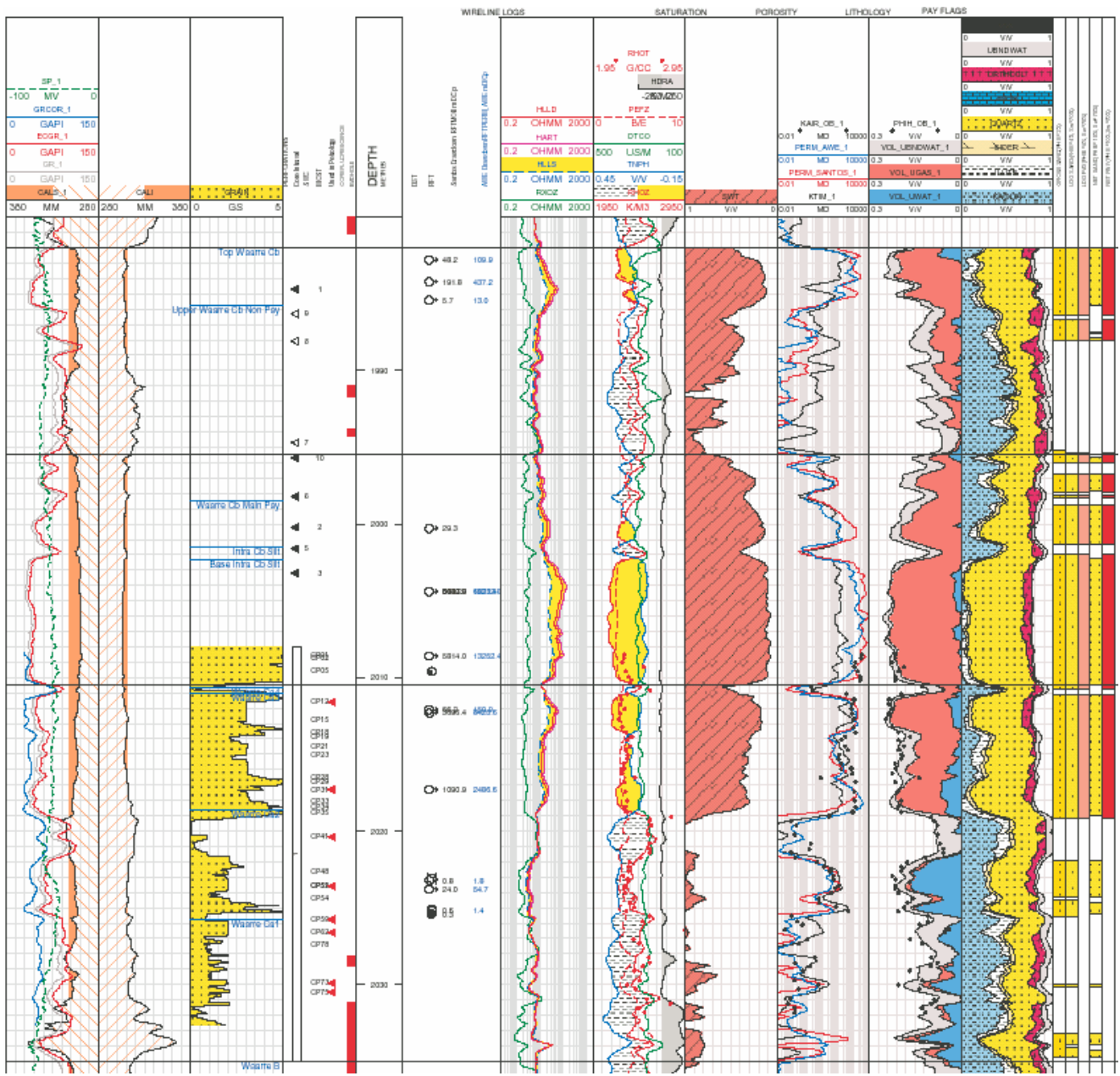
Figure 3.6.4 – e : Casino-3 Log Analysis (Waarre C Reservoir)
