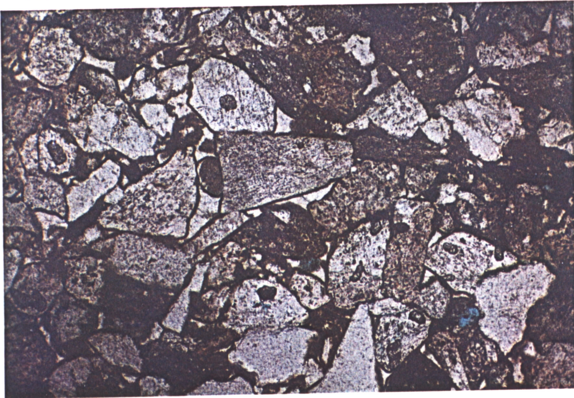
PHOTO 3 WIND. 2 1783M WELL SORTED LITHIC ARKOSIC ARENITE SHOWING STAINED CLAY RIMS AND CLEAR ?ZEOLITE CEMENT. NIC UNC. FIELD WIDTH 1.8MM
