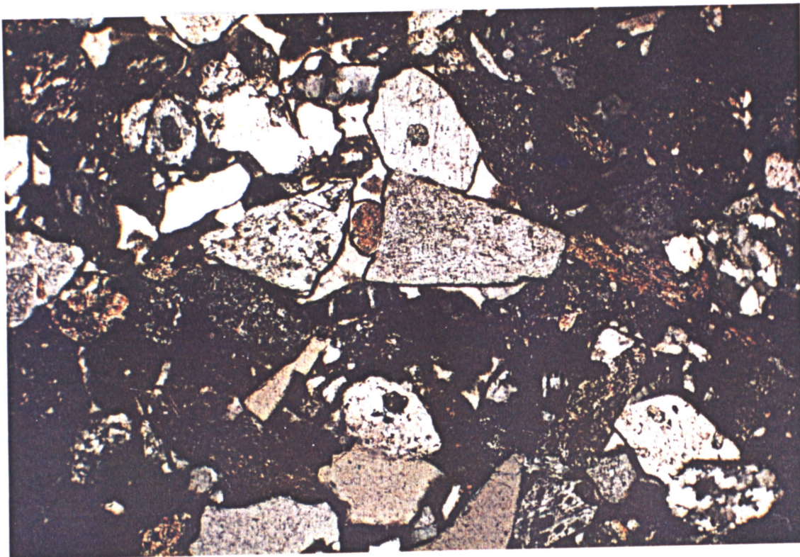
PHOTO 4 WIND. 2 1783M AS FOR PHOTO 3, SHOWING HETEROGENEOUS NATURE OF CLASTS. NIC CROS. FIELD WIDTH 1.8MM
