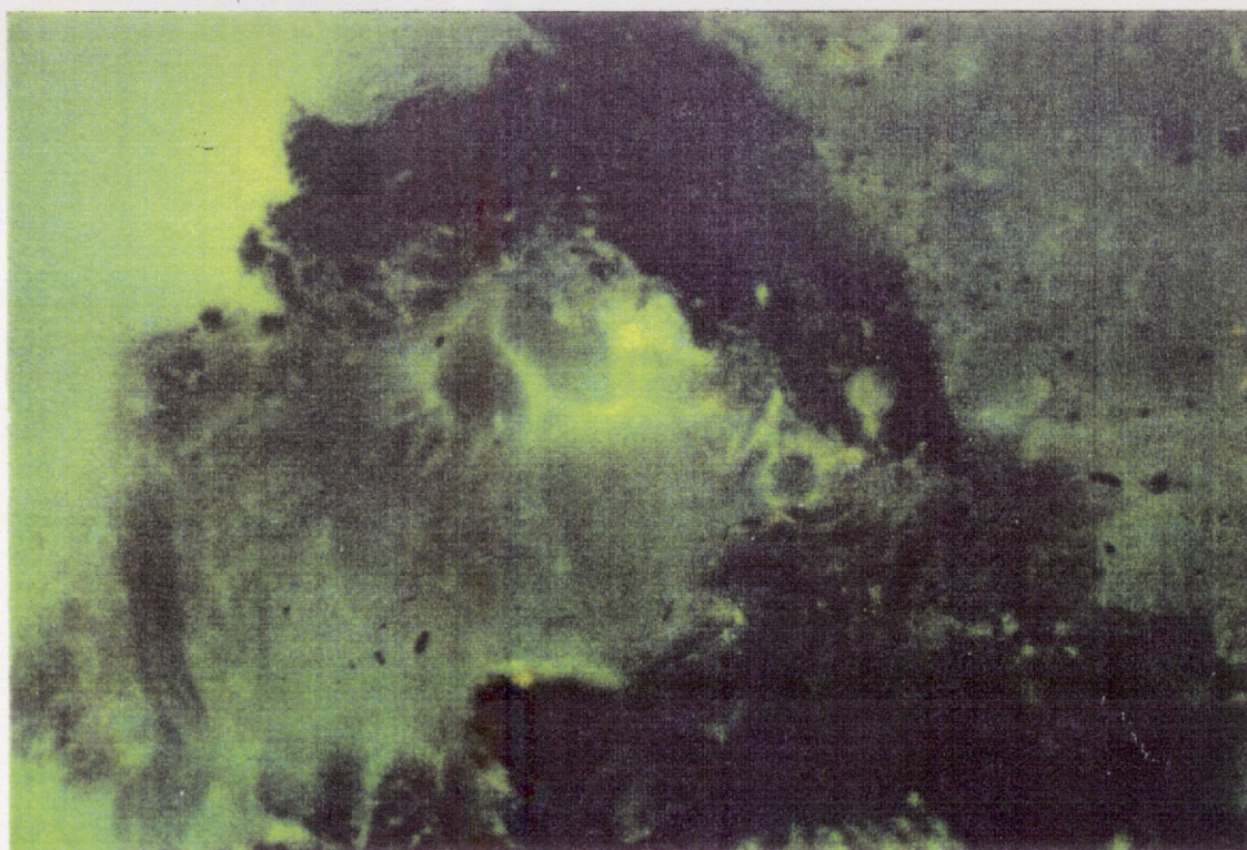
Plate 4: Same field as above Fluorescence Mode Oil (intense yellow green) is closely associated with the bituminite and vitrinite in this siltstone suggesting that this oil may have been generated "in situ" from this bituminite.
