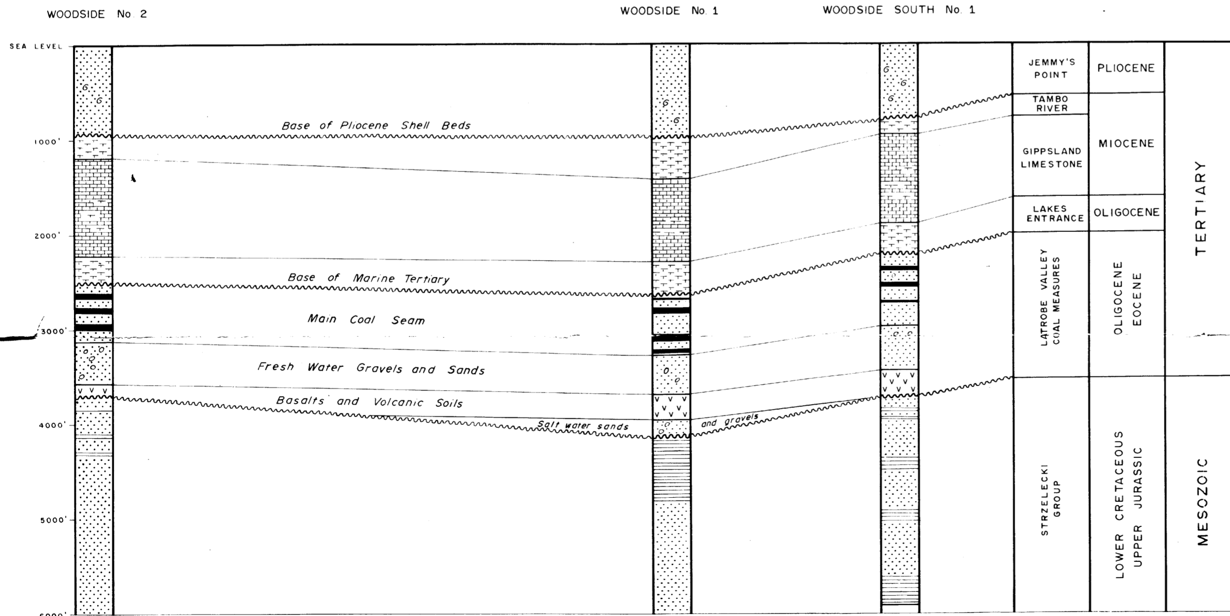
SECTION AFTER DRILLING WOODSIDE SOUTH No. 1
