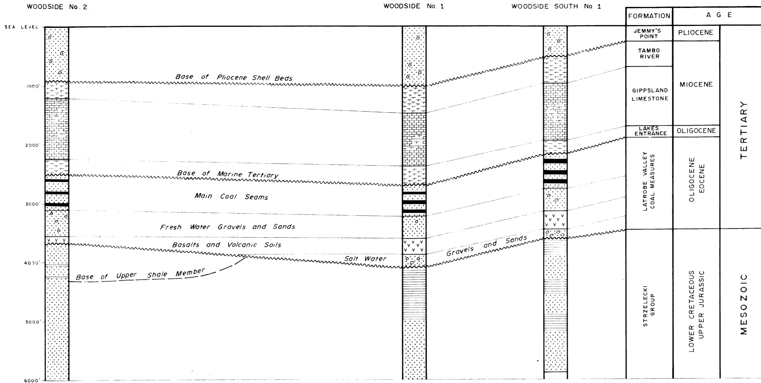
SECTION BEFORE DRILLING WOODSIDE SOUTH No. 1
