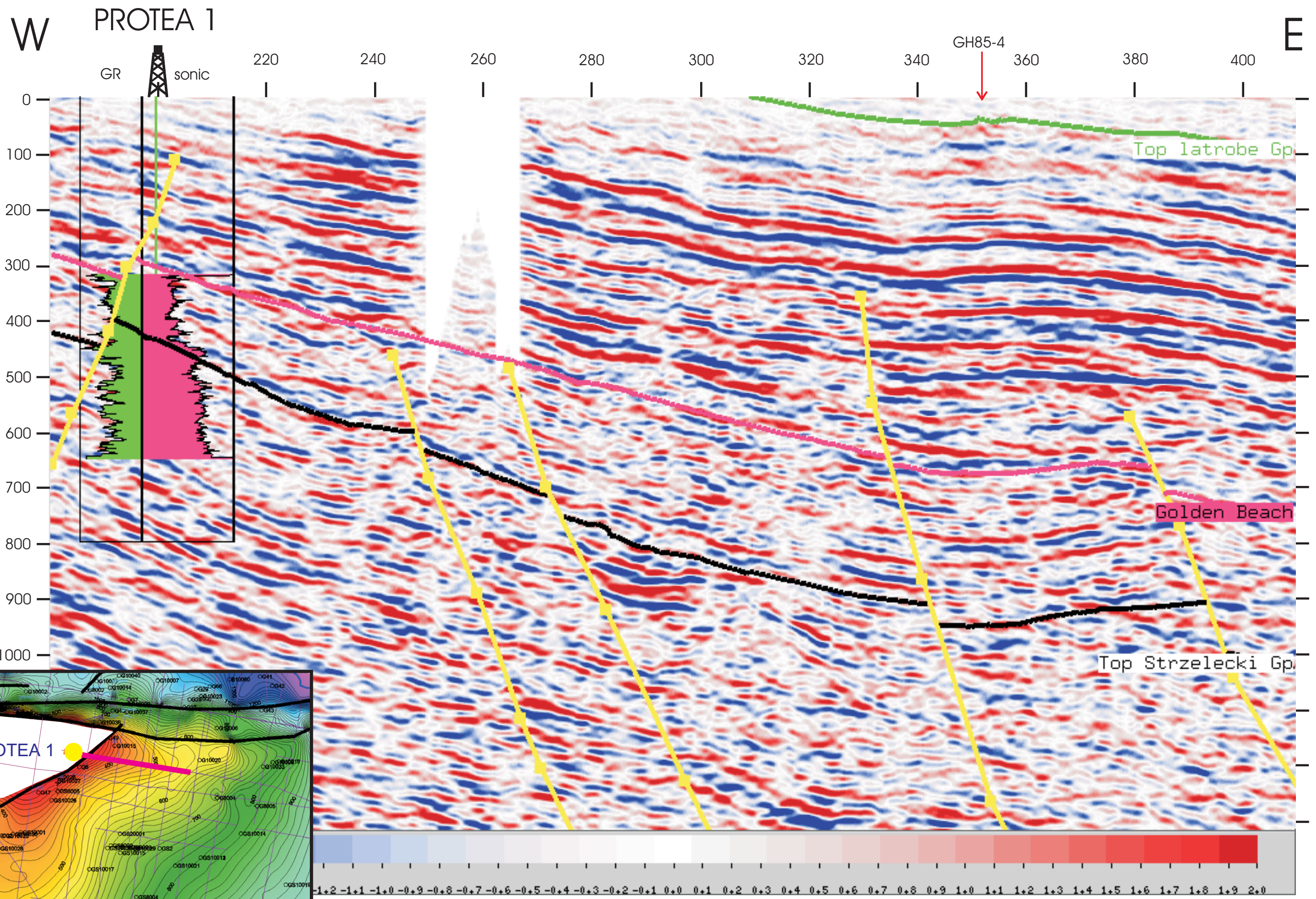
PROTEA 1 SEISMIC SECTION GCRP91A-12
