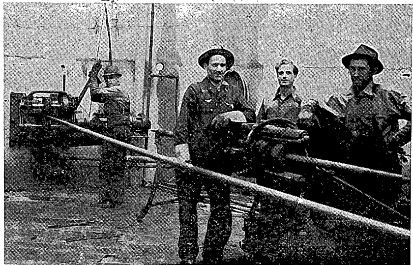
"Drilling two wells at a time". Pulling 50 feet of core from one well while running another set of tools and the drill rods into the opposite well. This is done by the newly developed "rod puller" which moves the tools at the rate of 100 feet per minute. Drill rods are not disconnected until both wells have been drilled to the desired length. Drilling machine is moved back (hydraulically) while tools are being moved. Compressed air motors are recommended as the best power for all machines in the work chamber.
