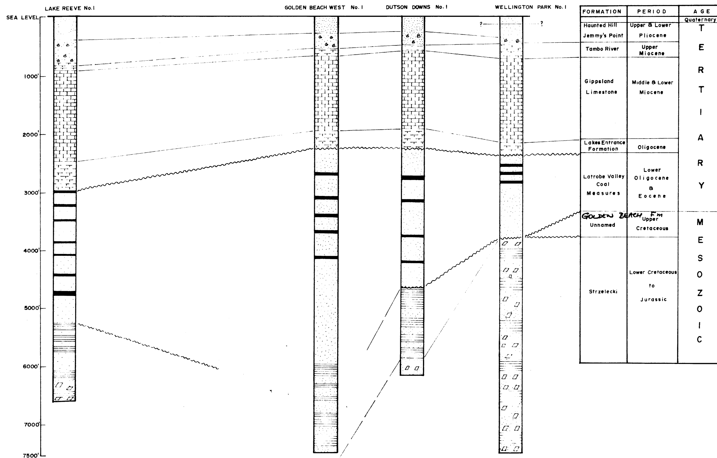
GEOLOGICAL SECTION AFTER DRILLING
