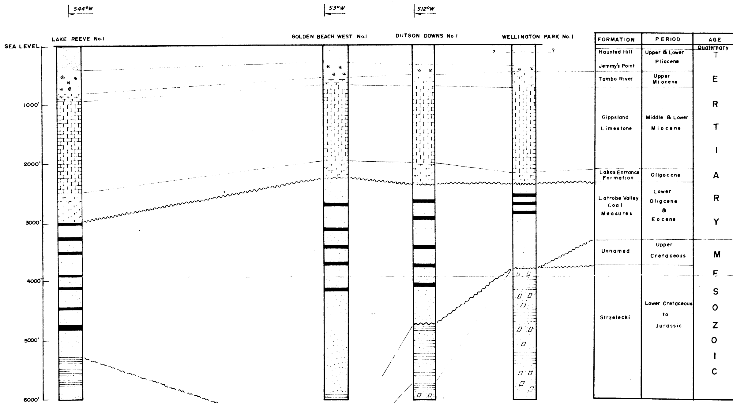
GEOLOGICAL SECTION BEFORE DRILLING
