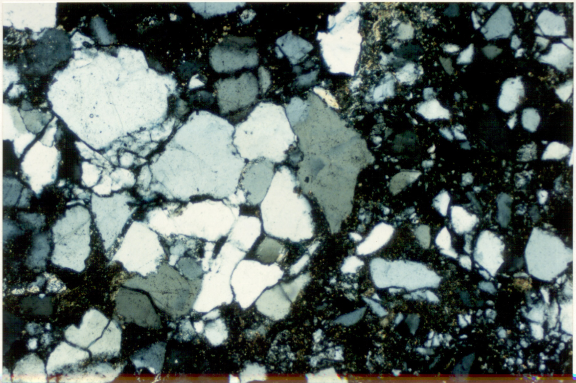
Figure 4: SWC 6, 3378m, 2mm, CL The right-hand side of the field shows typical damaged (fractured) material with a fine-grained "matrix". On the left is better-preserved, more siliceous sandstone which shows numerous long and concavo-convex boundaries.
