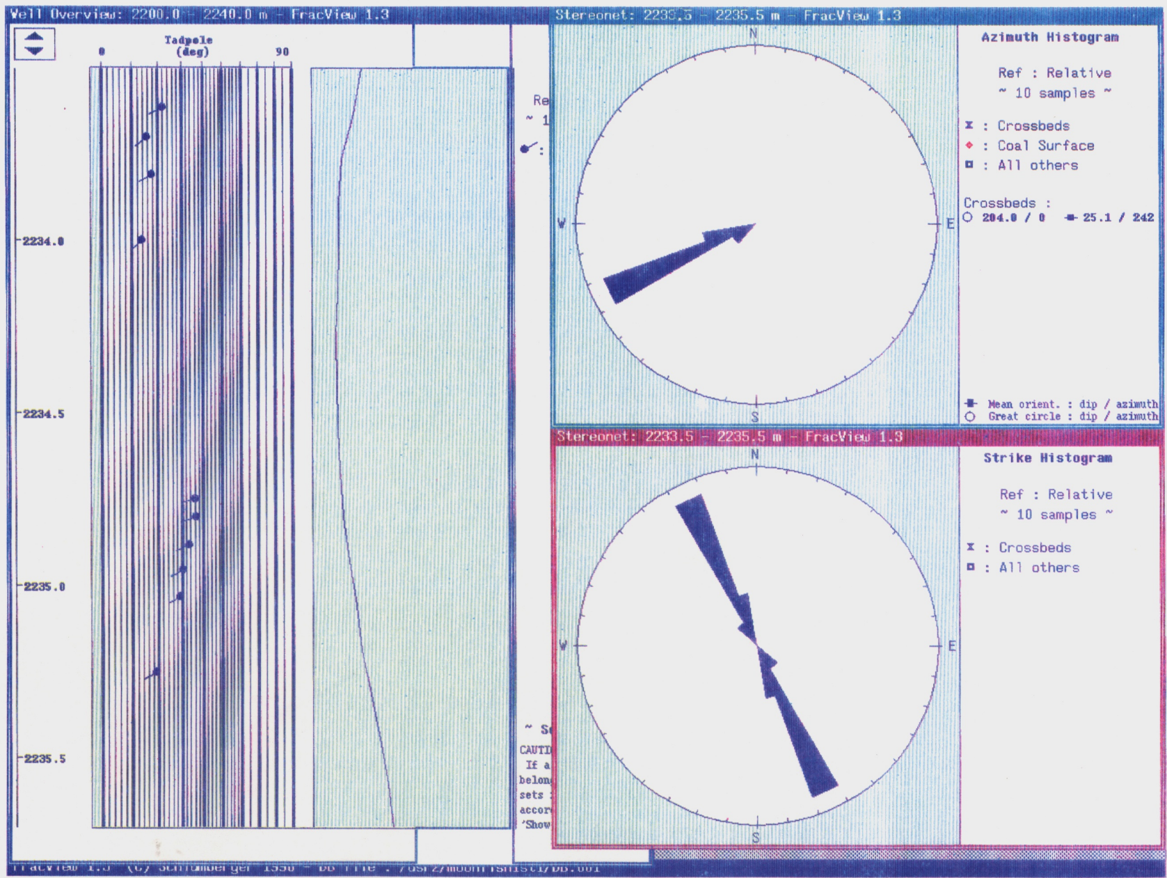
FIGURE 19 Crossbeds SDR Dip Azimuth 242° Interval 2233.5m to 2235.5m.
