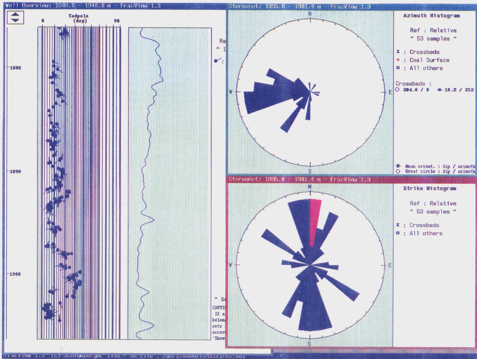
FIGURE 9 Crossbeds SDR Dip Azimuth 252° Interval 1895m to 1901.5m.
