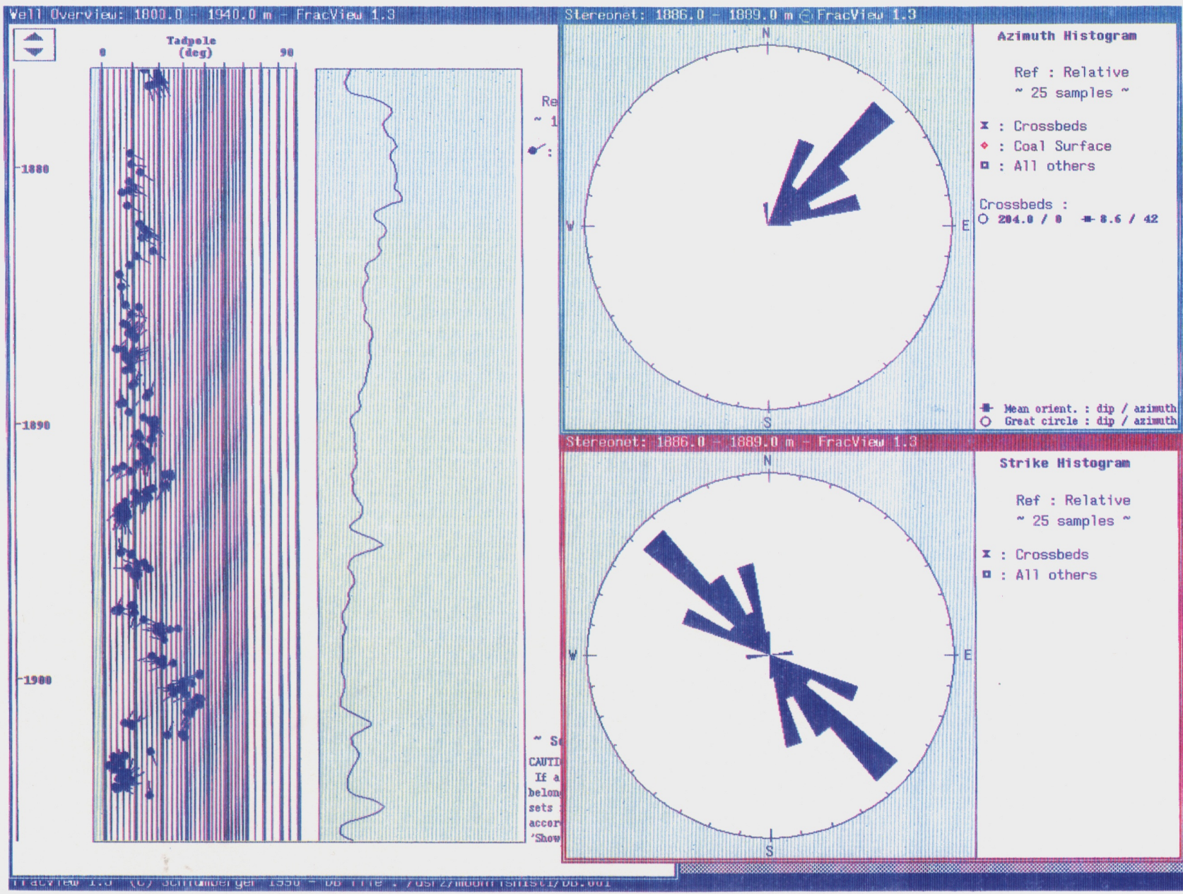
FIGURE 7 Crossbeds SDR Dip Azimuth 42° Interval 1886m to 1889m.
