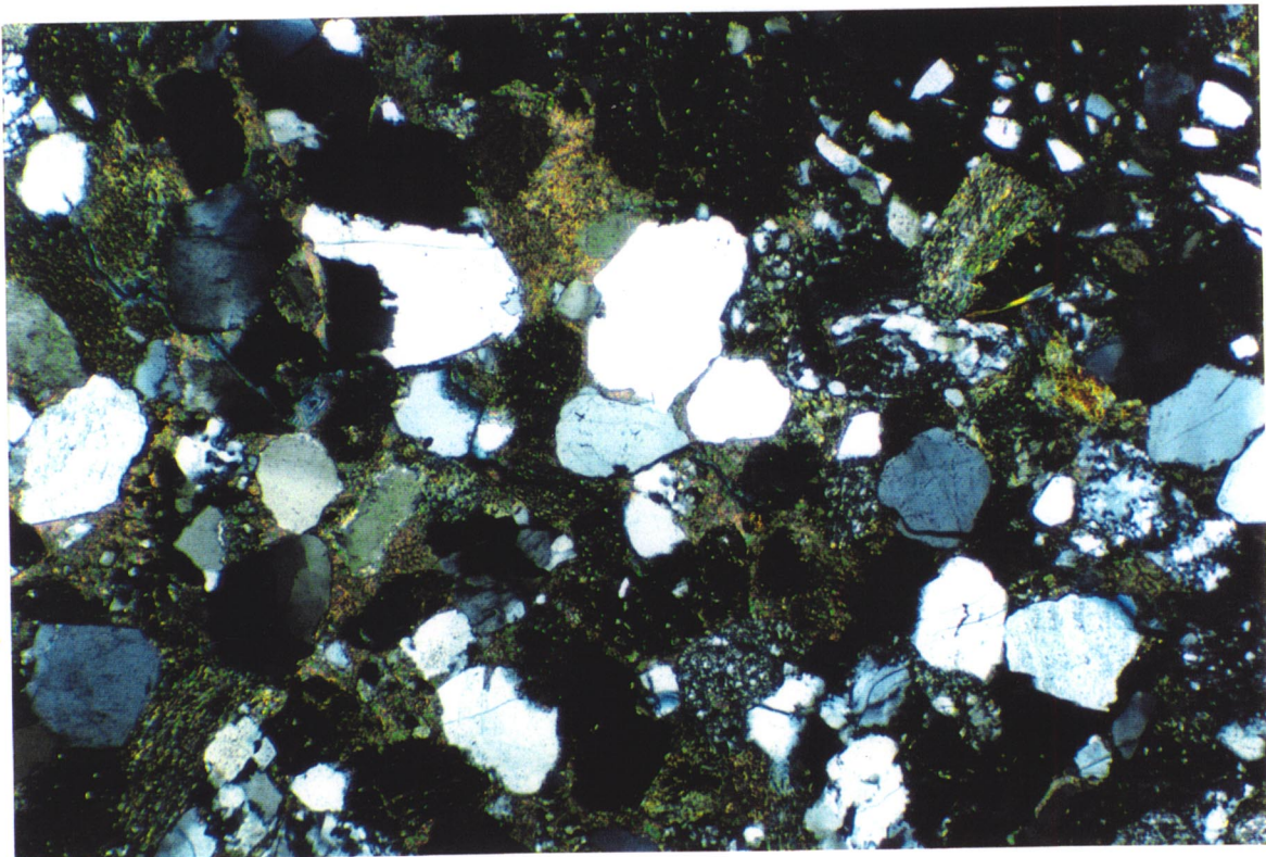
Figure 10: Sample 22 (1928.5 m): Plain (upper) and cross-polarised (lower) photomicrographs of calcite-cemented litharenite. Poikilotopic calcite (speckled pinky brown) is pervasive and completely occludes porosity. This sample is relatively uncompacted which suggests that calcitization occurred during early diagenesis. Fractures are sampling induced. Long axis of photomicrograph is equal to 2.72 mm.
