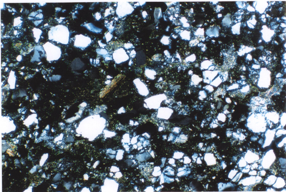
Figure 8: Sample 25 (1911.0 m): Plain (upper) and cross-polarised (lower) photomicrographs of litharenite. Note extensive sampling-induced damage. Note compacted lithic grains (L). Long axis of photomicrograph is equal to 2.72 mm.
