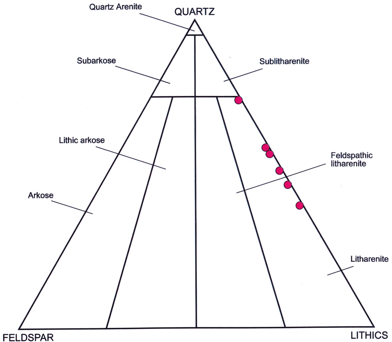
Figure 1: Folk (1964) classification scheme showing position of Longtom-1 samples (red dots). Classification involves the removal of matrix, mica and cement and recalculation of components (quartz, feldspar and lithics) to 100%.
