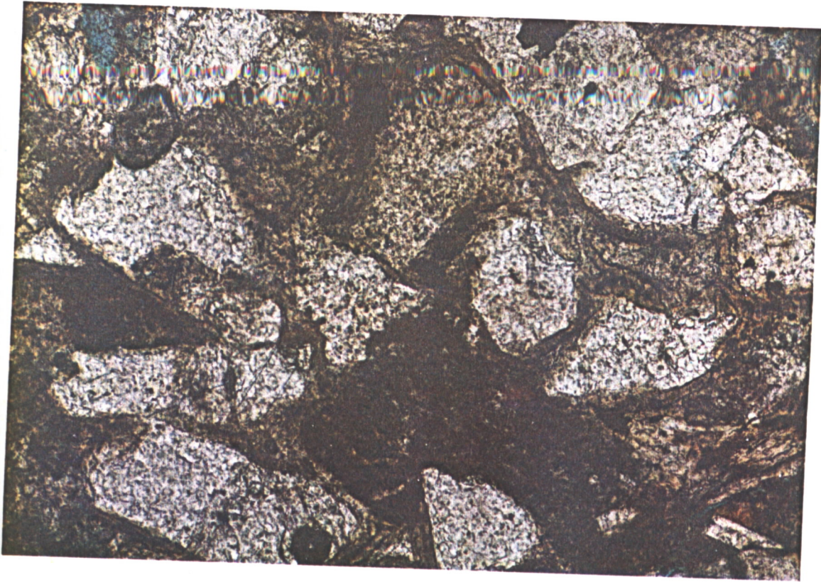
PHOTO 11 WIND. 2 3190M CLAY RIMMING AND CEMENTING WELL SORTED LITHIC ARKOSIC ARENITE. NIC UNC. FIELD WIDTH 0.7MM
