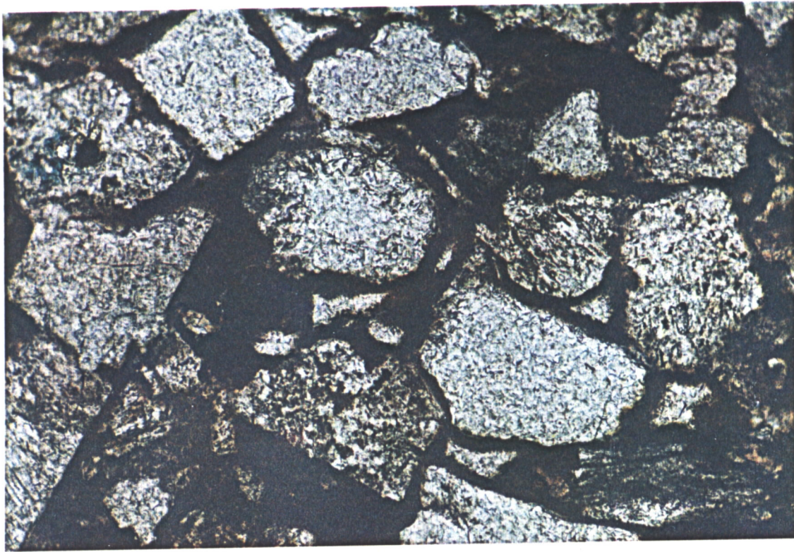
PHOTO 2 WIND. 2 1746M QUARTZ/FELDSPAR/LITHIC CLASTS RIMMED BY STAINED CLAY MATRIX, PLUS CLEAR ?ZEOLITE CEMENT. NIC UNC. FIELD WIDTH 0.7MM
