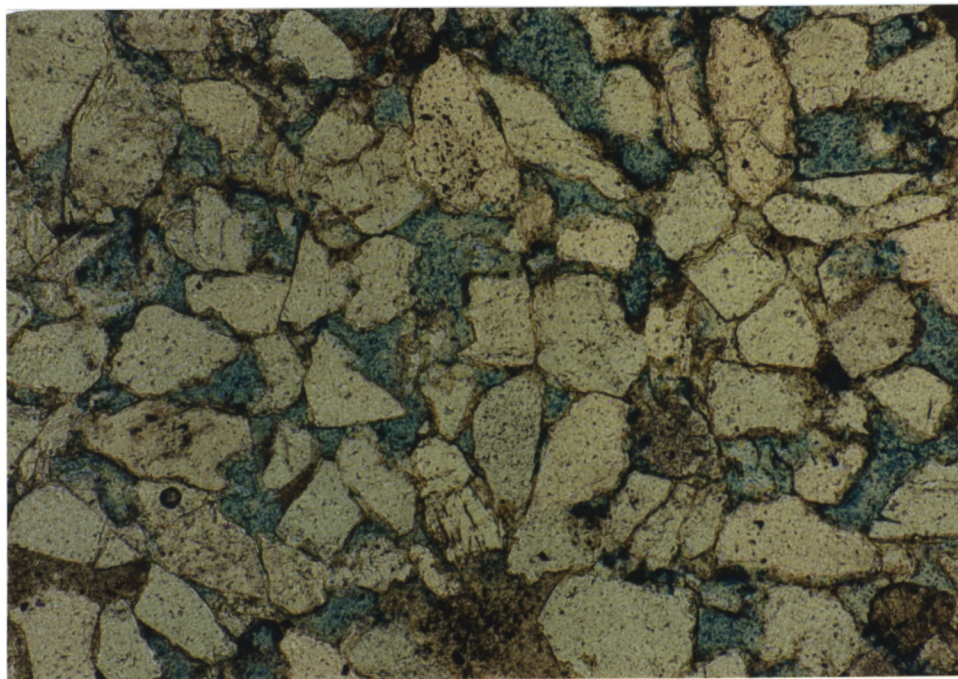
FIGURE 2b: 1814.5 m Plane polarised light (2 mm). Typical view. Blue-stained pores are abundant. A little brown clay is present in patches and as a film on some grains.
