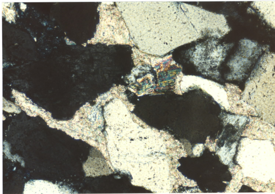
FIGURE 2a: 1814.5 m Crossed Nicols (1 mm). Quartz grains embedded in single crystal of carbonate (speckled buff colour) which locally occludes all porosity. A corroded muscovite flake (centre, bright colours) is also shown.
