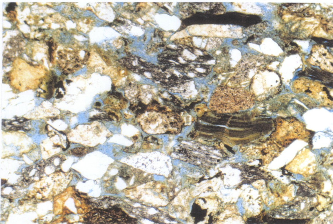
Figure 4a General view showing an open framework of well sorted sand grains. Tangential and point contacts are common. Green chlorite lines all pores. Swc 9, depth 1426m. Plane light. Field of view 2.5mm.
