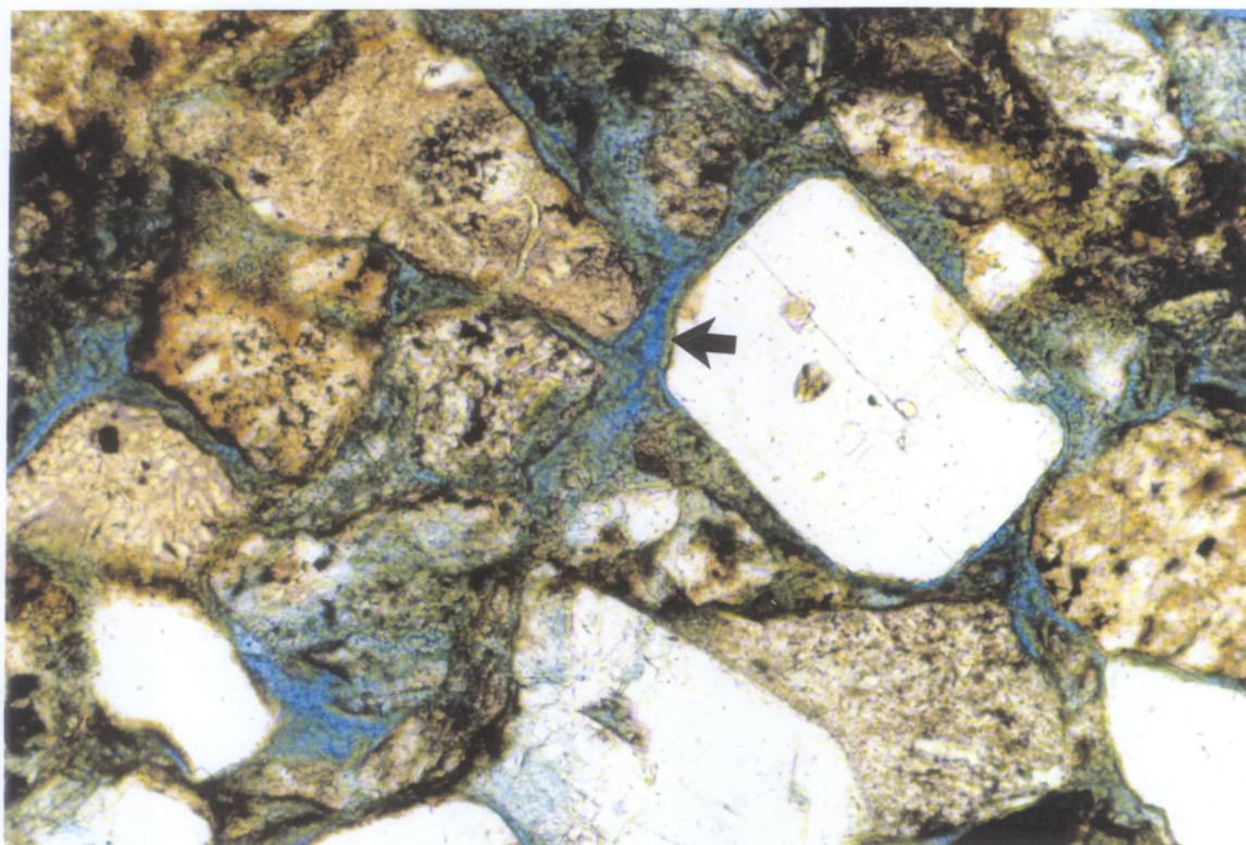
Figure 4b Lithic grains are generally smaller than the feldspar. The lithic grains are generally undeformed and are cemented with rims of green chlorite (arrow). Swc 9, depth 1426m. Plane light. Field of view 1mm.
