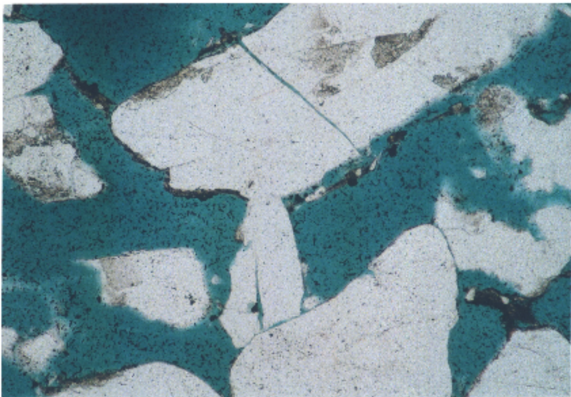
Plate 12: Sample # 2 (1307.50m) Thin section photomicrograph showing traces of infiltrated drilling mud filling some of the pore spaces and coating some of the detrital grains. Plane polarised light. Scale bar = 200 \mu m.
