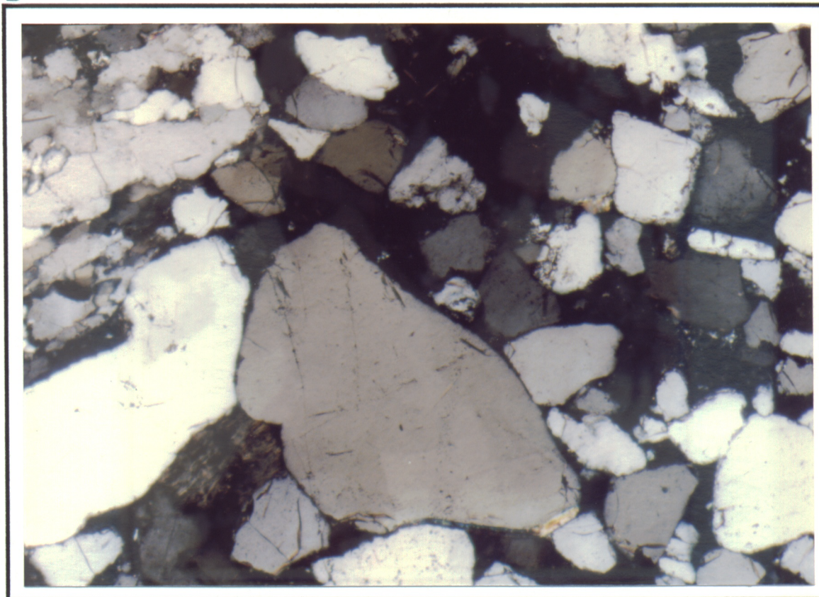
Figure 3: GC333-3, Omeo-1, Core 1. Latrobe Group quartz sandstone. Framework dominantly rounded to sub-angular granitic quartz with large variation in grain size, some "fresh" orthoclase and muscovite. Unstable lithic grains and polycrystalline quartz of low abundance. 1° porosity abundant, 2° porosity in K-feldspar. A . Plane polarised light Width of field of view = 2.20 mm B . Crossed polarised light Width of field of view = 2.20 mm
