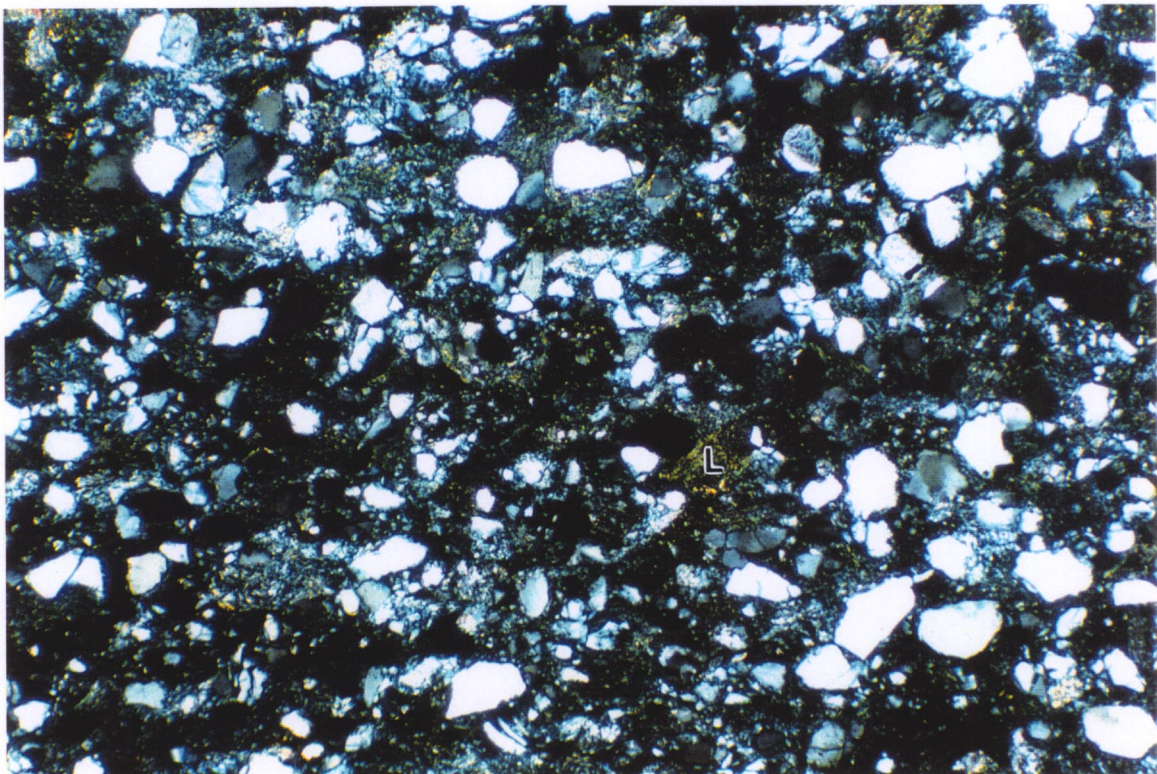
Figures 9: Sample 23 (1923.5 m): Plain (upper) and cross-polarised (lower) photomicrographs of litharenite. Deformed lithics (L) are abundant. Relict porosity is partly occluded by kaolinite (K). Long axis of photomicrograph is equal to 2.72 mm.
