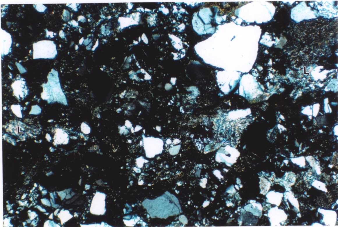
Figure 7: Sample 26 (1904.5 m): Plain (upper) and cross-polarised (lower) photomicrographs of litharenite. Grain disaggregation occurred during sampling. Nevertheless, fragments of deformed lithics (L) are abundant and indicate that porosity was probably destroyed due to extensive compaction. Long axis of photomicrograph is equal to 2.72 mm.
