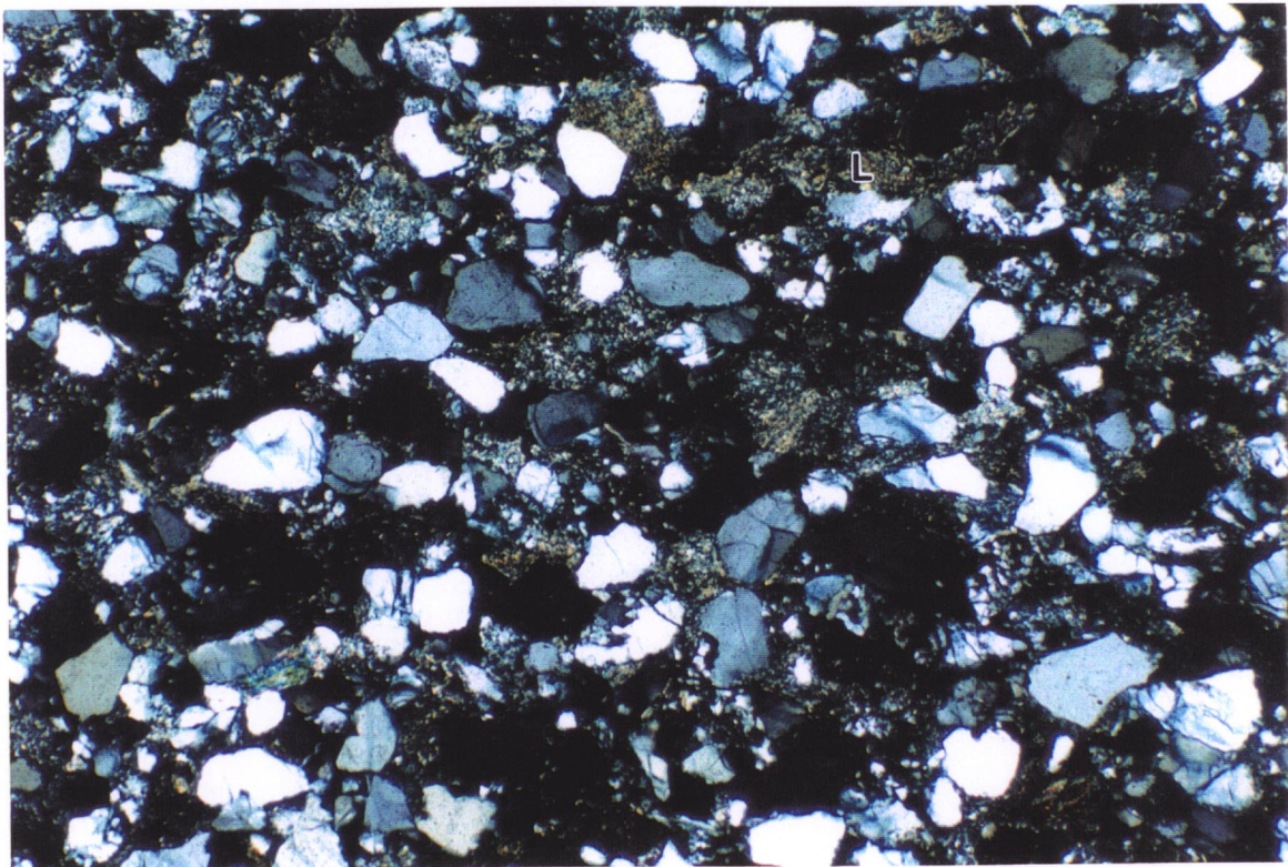
Figure 6: Sample 27 (189.5 m): Plain (upper) and cross-polarised (lower) photomicrographs of litharenite. Fractures result from impact-damage. Note abundant ductily deformed lithic grains (L). Porosity (light blue) is partly occluded by kaolinite and difficult to estimate due to sampling-induced changes in grain packing. Long axis of photomicrograph is equal to 2.72 mm.
