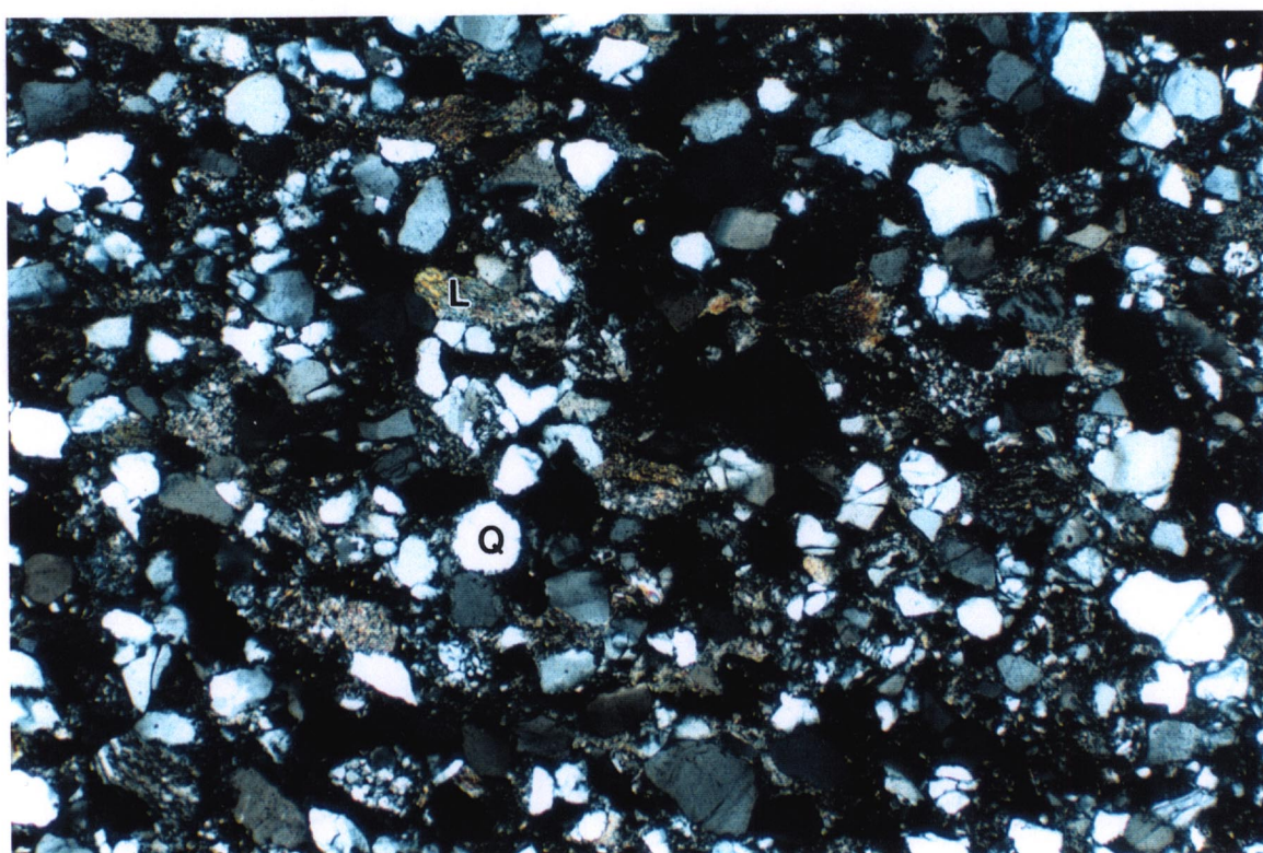
Figure 2: Sample 28 (1892.5 m): Plain (upper) and cross-polarised (lower) photomicrographs of litharenite. Sample disaggregation has resulted from impact damage. Note abundant lithic (L) and detrital quartz (Q) grains. Kaolinite (K) occludes some pores. Long axis of photomicrograph is equal to 2.72 mm.
