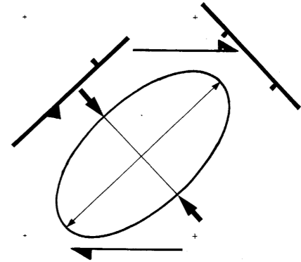
NOTIONAL REGIONAL STRAIN CAUSED BY DEXTRAL SHEAR AND RELATIONSHIP TO SECONDARY NORMAL AND REVERSE FAULTS.
