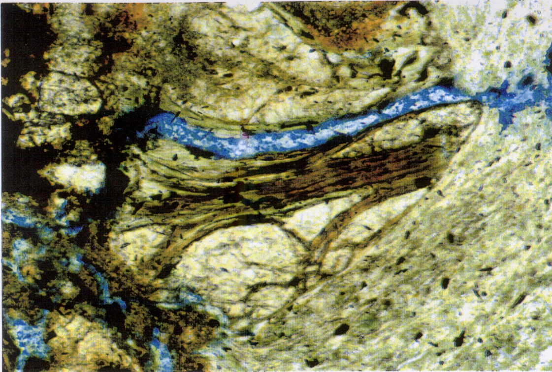
Figure 3. The displacive influence of carbonate cement is demonstrated by this splayed biotite. Chlorite (pale green) has selectively replaced some flakes of the biotite. Opaques concentrating along these flakes are probably reaction products of this alteration. Blue dye highlights fracturing caused by sidewall collection. Devilfish #1, sidewall core 2, depth 2020m. Plane light. Field of view 0.45mm.
